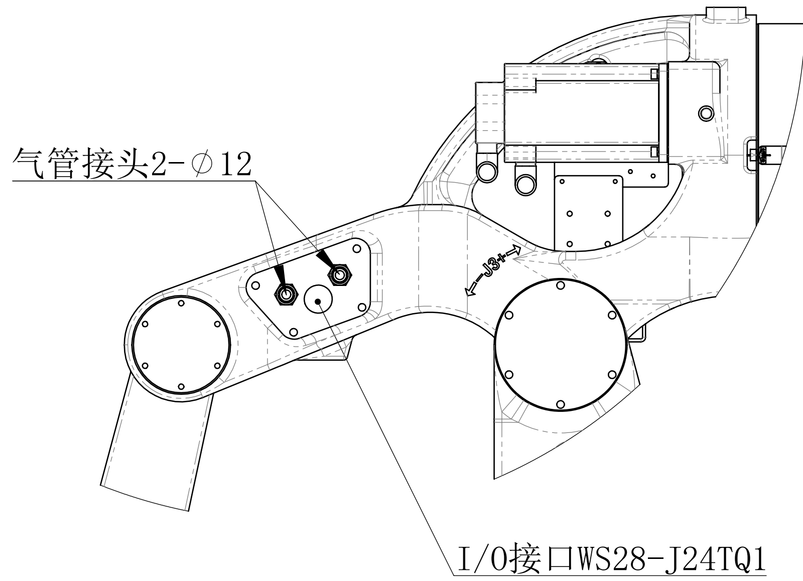
I/O接口WS28-J24TQ1
